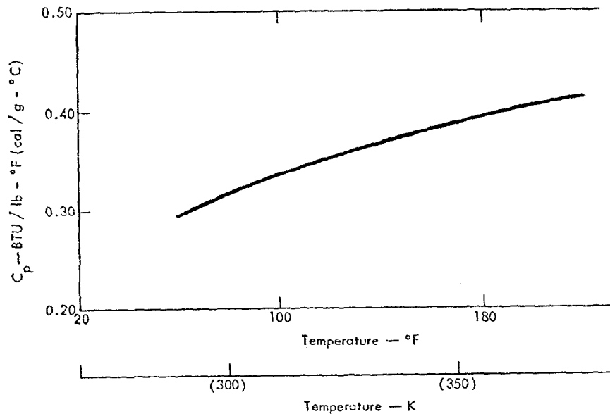
Fig 1 Specific heat C_p of RDX as a function of temperature. Conversion 1 \text{ BTU/lb}\cdot\text{°F} = 1 \text{ cal/g}\cdot\text{°C} = 4.184 \text{ kJ/kg}\cdot\text{K}
